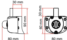
Safe Door Guardian Ducato > 2009
